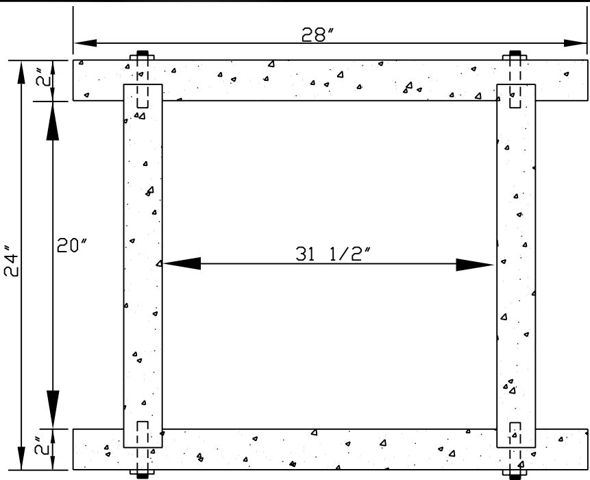
PLAN
