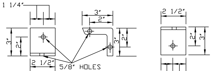
3"X3" STD. 3/8" ANGLE
